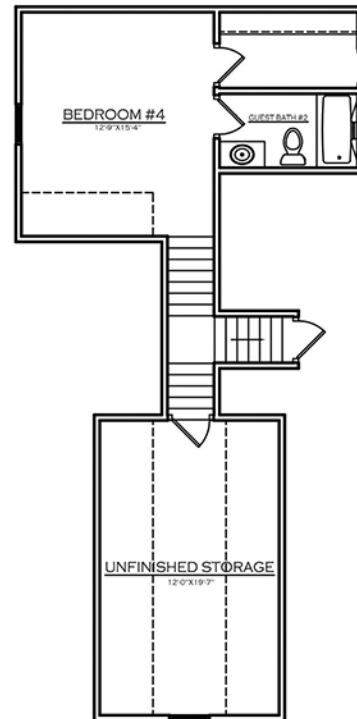
Optional 2 nd Floor (2,358 sq. feet)
