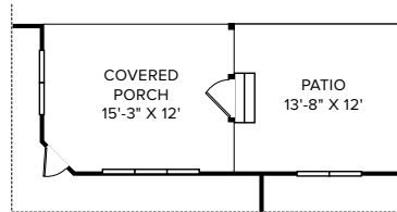
OPT. COVERED PORCH
