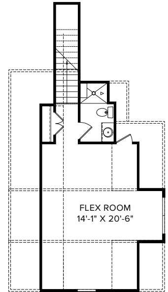
FLEX ROOM B 422 Sq. Ft.
